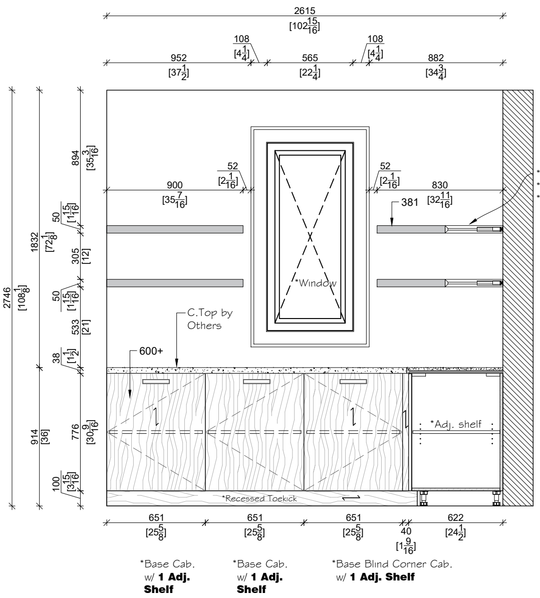
*PANTRY ELEVATION
