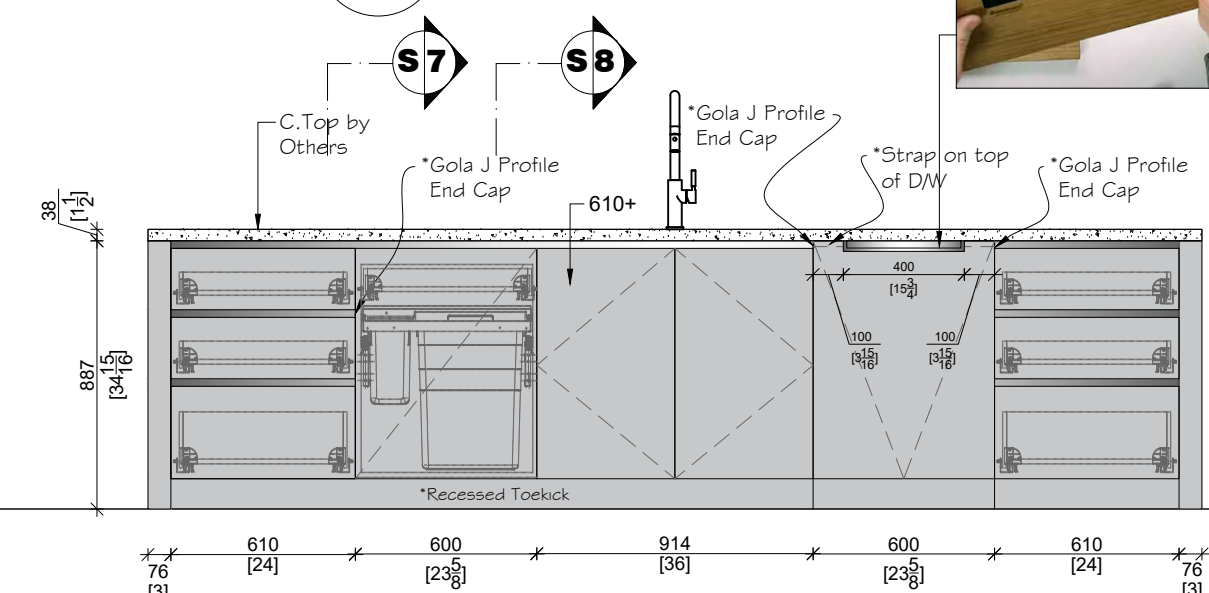
H - View of Island SCALE: 1:25
