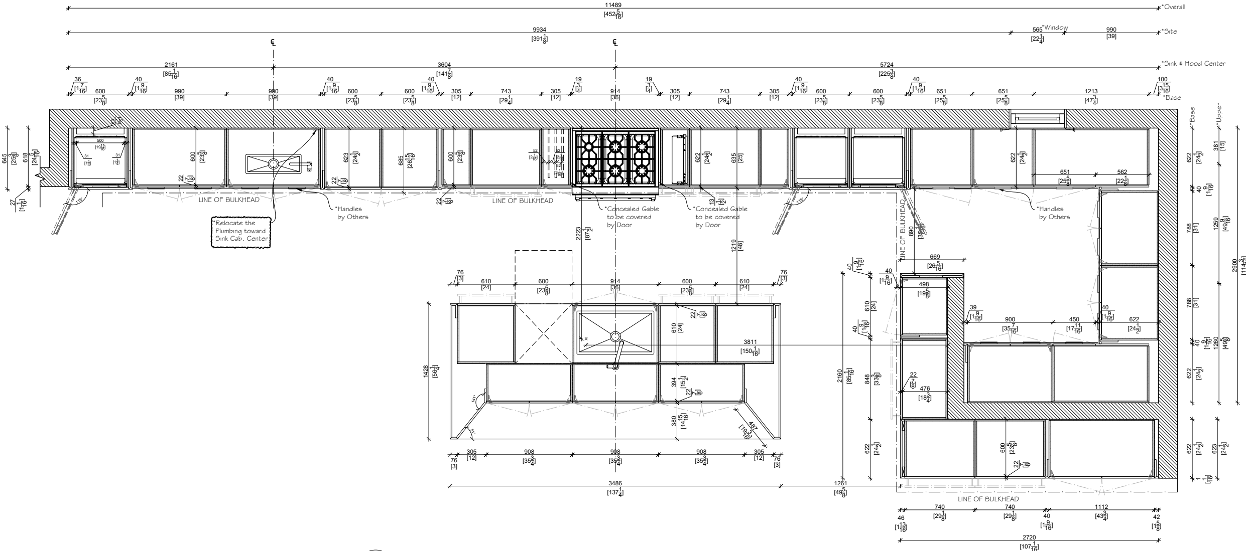
PLAN - BASE LAYOUT SCALE: 1:40 * Existing Hot & Cold Water Pipes * Existing Drainage
